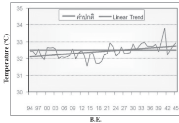
Average annual maximum temperature trend in Thailand
